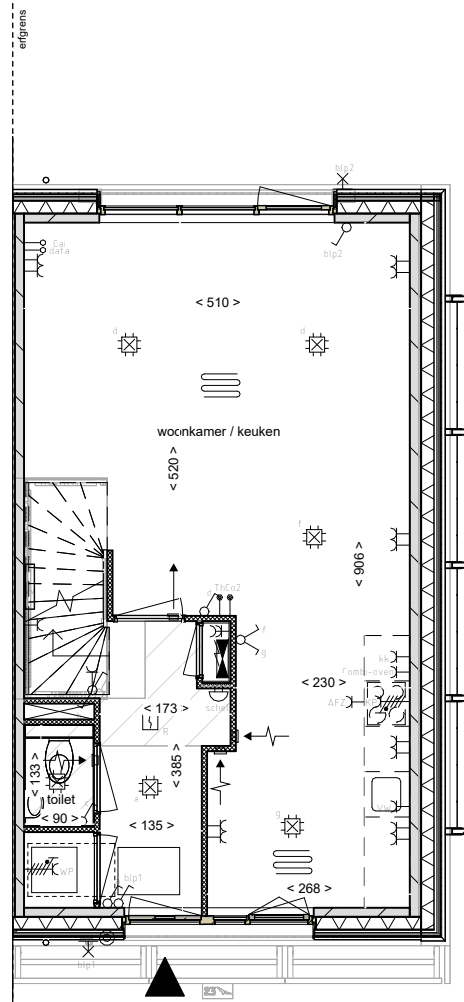
00 begane grond
